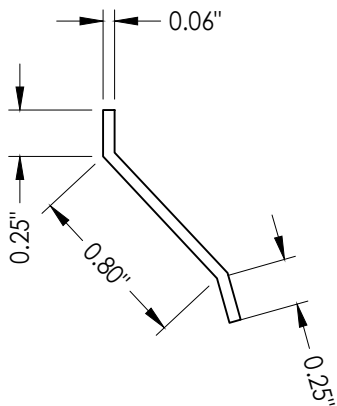
90 STEEL LOUVER
